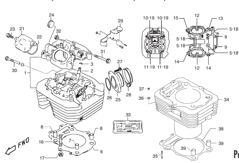
TAV.2 Testa-cilindro - Cylinder head - Culasse - Zylinderkopf - Culata
