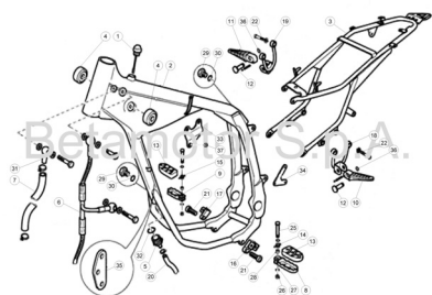
TAV.31 Telaio - Frame - Chassis - Rahmen - Chasis
