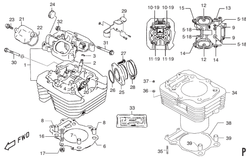
TAV.11A Testa-cilindro - Cylinder head - Culasse - Zylinderkopf - Culata
