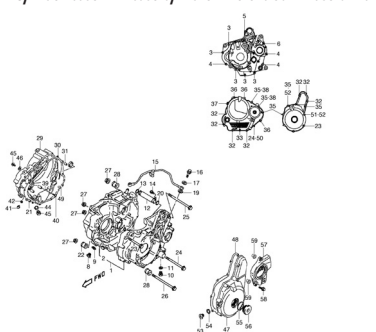
TAV.01 Basamento - Cylinder base - Embase cylindre - Motorblock - Base cilindros
