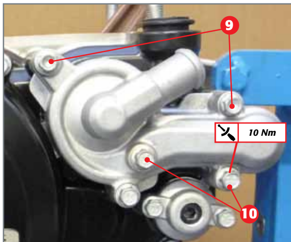
Pumpendeckel.
